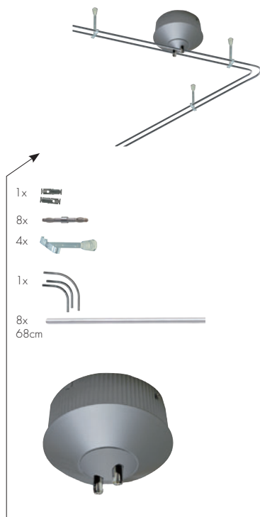
Basic Bogen 150 max. 150W 230/12V, 150VA ⚡ ⇄280cm ⇄30mm EAN 4000870 054123 5412
