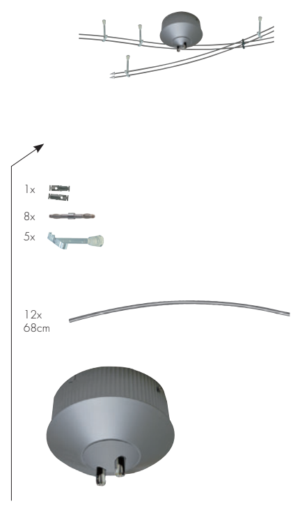
Basic Hip Hop 200 max. 200W 230/12V, 210VA ⚡ ⇄210/140cm ⇄30mm EAN 4000870 054109 5410
