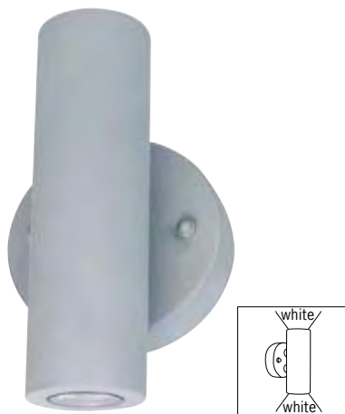
Facula incl. 2x1W 230V ø90 ⇄100 ⇄172mm EAN 4000870 997789
